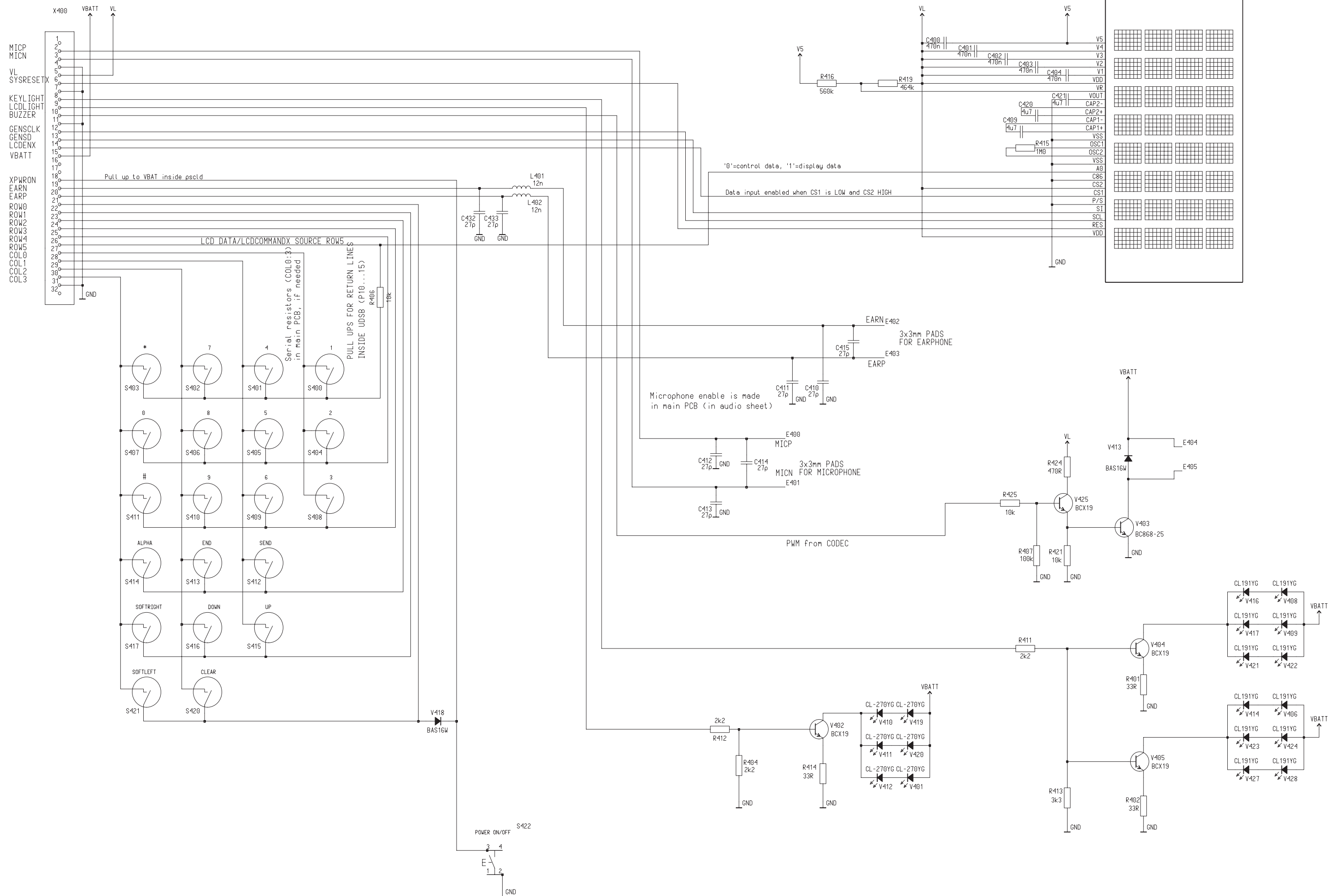
Figure 5 UIF Schematic
